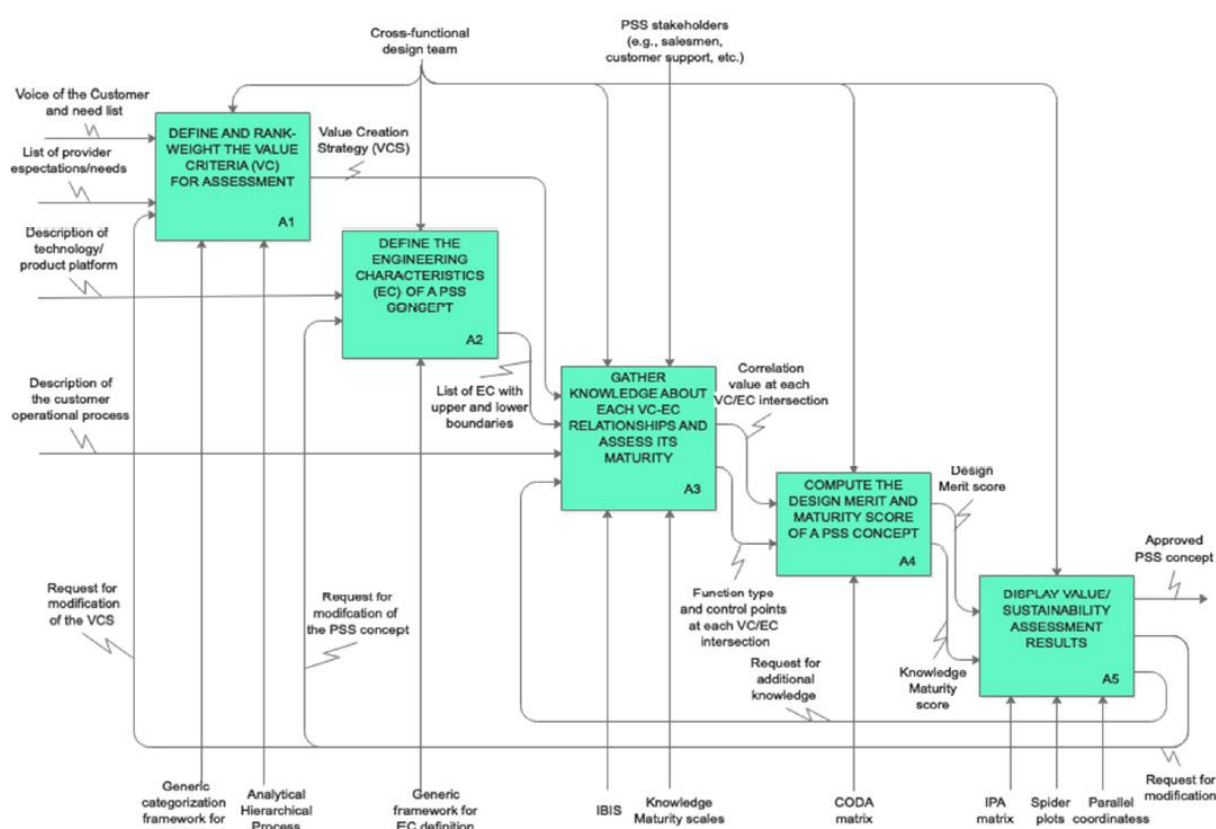
Slika 7 Koraci MCDM for Sustainability and Value Assessment metode [16]
